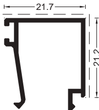
COD 1.36 G=0.25 kg/m P=159 mm Bagheta 21,7mm
