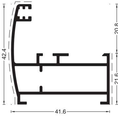
COD 1.25 G=0.67 kg/m P=256 mm Toc mic
