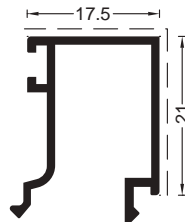
COD 1.41 G=0.24 kg/m P=154 mm Bagheta 17,5mm
