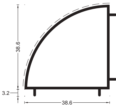
COD 1.32 G=0.48 kg/m P=162 mm Adaptor 90°
