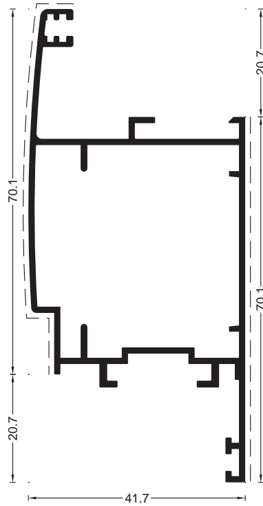
COD 1.43 G=1.03 kg/m P=370 mm Cercevea medie
