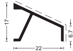
COD 1.42 G=0.18 kg/m P=94 mm Picurator
