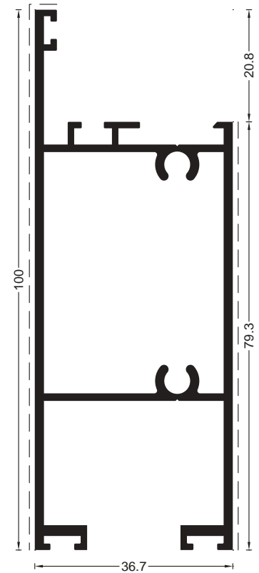
COD 1.19 G=1.41 kg/m P=435 mm Bandou
