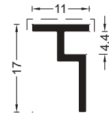
COD 1.37 G=0.22 kg/m P=121 mm Bagheta 5,2mm
