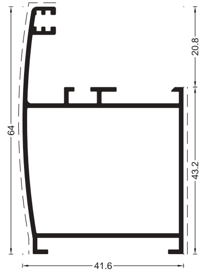
COD 1.19 G=1.41 kg/m P=435 mm Bandou
