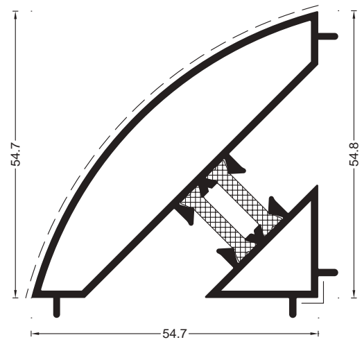
COD 2.18 G=1.24 kg/m P=324 mm Adaptor 90°
