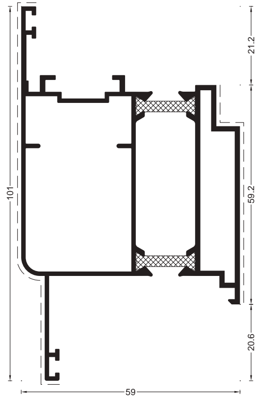
COD 2.18 G=1.24 kg/m P=324 mm Adaptor 90°
