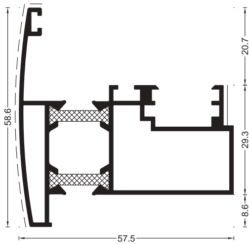
COD 2.16 G=1.18 kg/m P=348 mm Inversor
